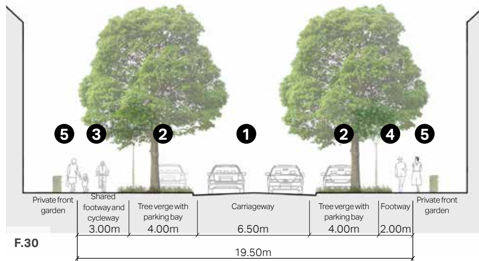
Figure 30: Section showing indicative dimensions for primary roads. In some places trees may be omitted from one or both sides although they help with placemaking, contribute to local biodiversity, and create a positive micro-climate
